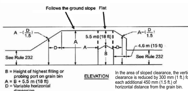
Figs. 234-4(b) Clearance Envelope for Grain Bins filled by portable augers, conveyors or elevators
